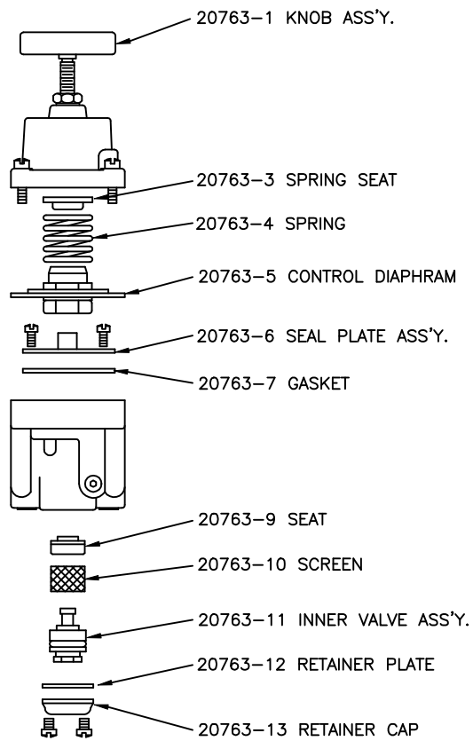
3/8"AIRBAG REGULATOR 20763
